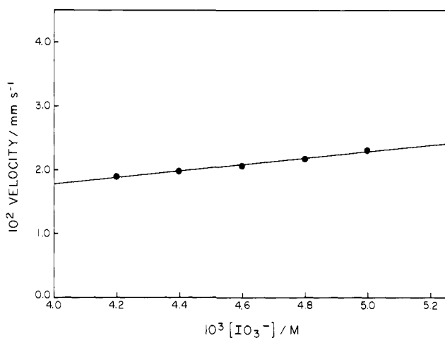
Figure 4. Wave velocity as a function of [IO_3^-]_0 in solutions containing excess arsenous acid. Solution compositions in Table I.
