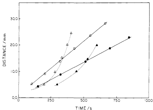
Figure 3. Wave front position as a function of time for reaction mixtures containing excess arsenous acid (solid lines) and excess iodate (dashed lines). Solution composition [X]_0 in Table I except [H_3AsO_3]_0 = 5.43 \times 10^{-2} M (O), 3.10 \times 10^{-2} M (●), 1.09 \times 10^{-2} M (Δ), 4.65 \times 10^{-3} M (▲).
